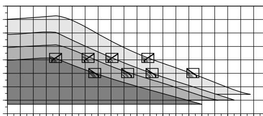
Fig. 15 UPM3 FLEX/HYBRID control modes with pump curves
