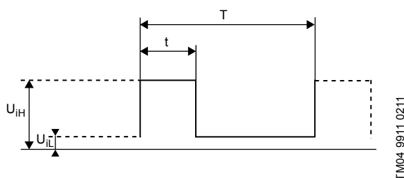
Fig. 4 PWM signal
